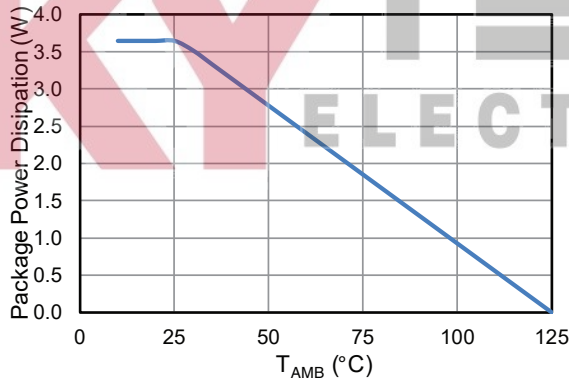
Figure 13: Package Derating
