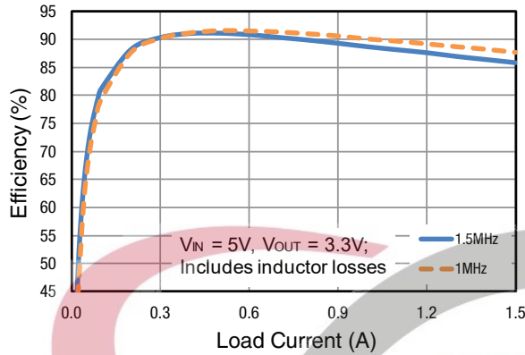
Figure 3: Buck 1 Efficiency
